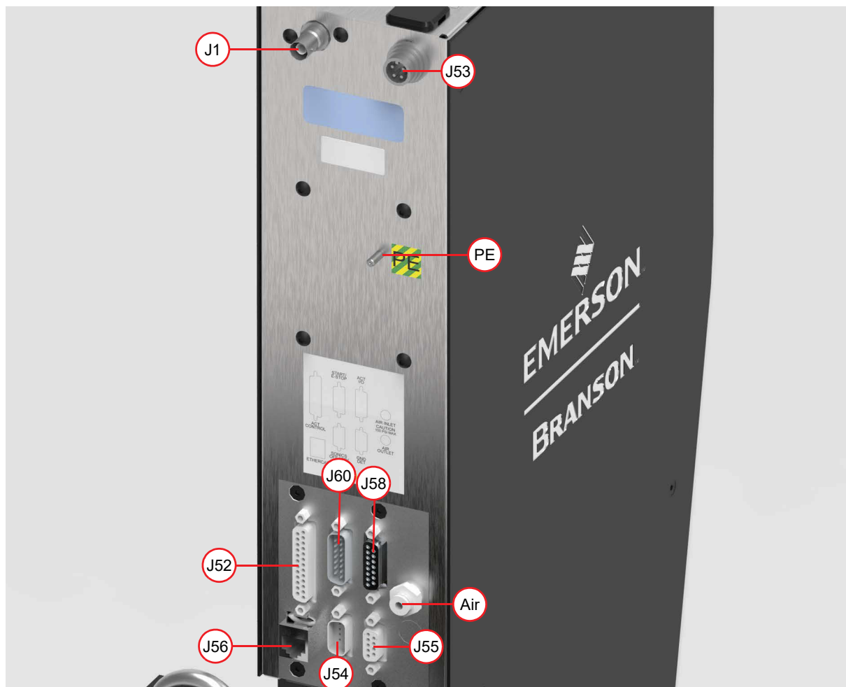
Figure 2.3 GSX Actuator Cable Interface Points
