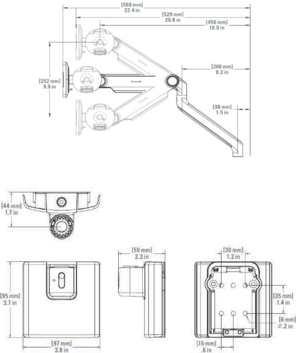
Figure 4.19 Dimensions - Monitor Arm
