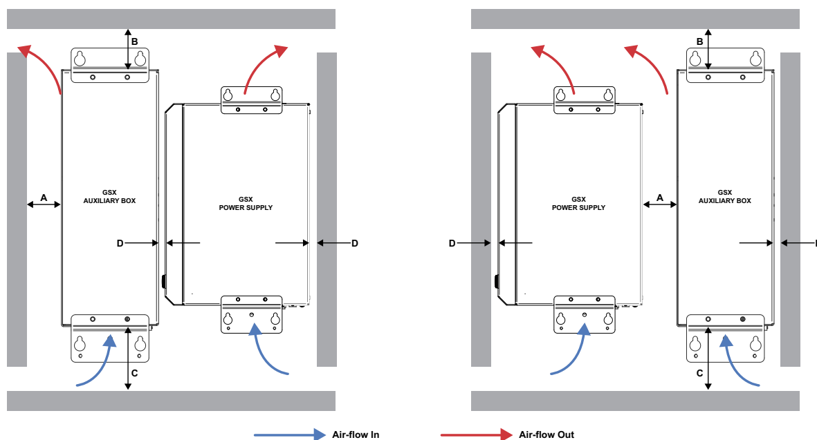
Figure 4.1 Air flow paths and clearances needed
