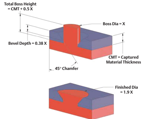
Figure 7. Flush Stake
